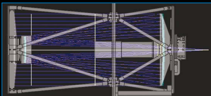
Optical Layout
